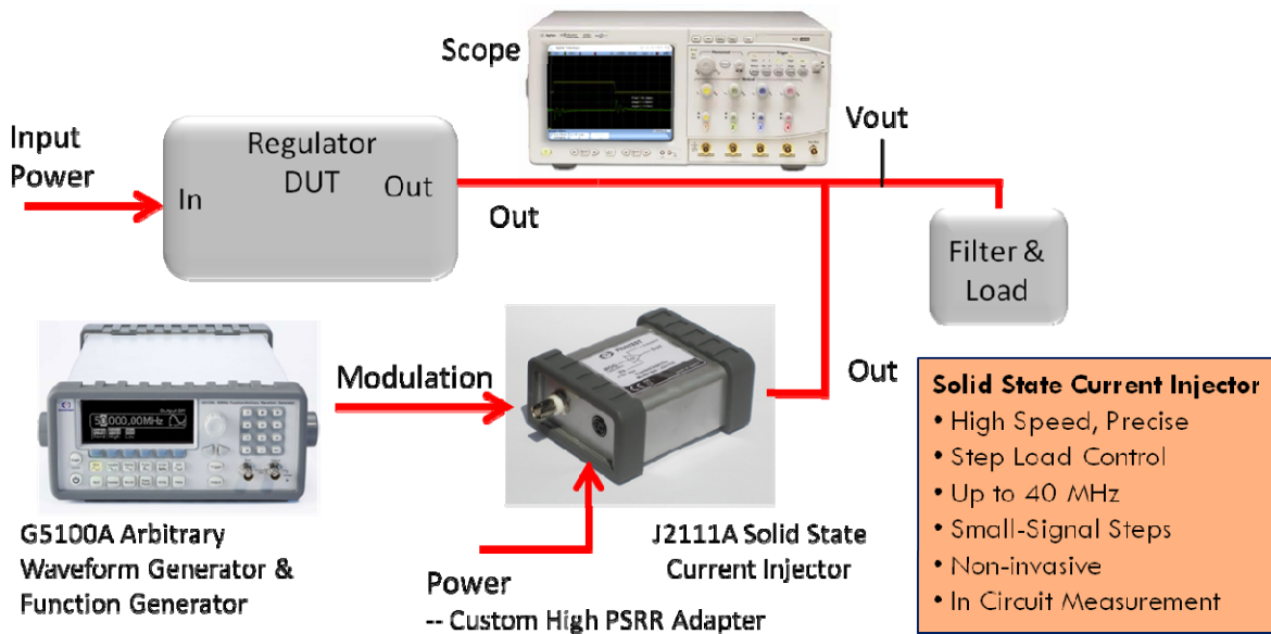
Figure 3 – Sample setup for the Solid State Current Injector (J2111A) used to perform a non-invasive load transient measurement.
