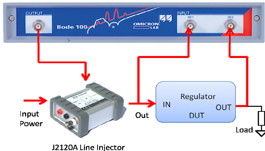
Figure 2 – Sample setup for the Line Injector (J2120A) used to perform a PSRR measurement
