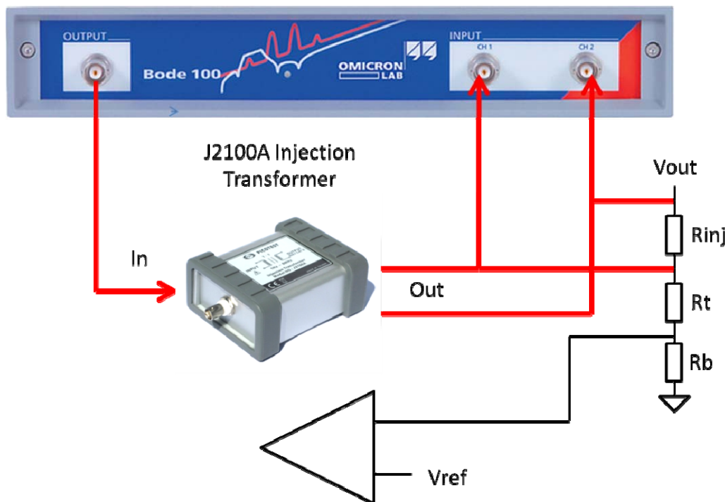
Figure 1 – Sample setup for the injection transformer (J2100A or J2101A) or the solid-state injector (J2110A) used to perform stability measurements.
