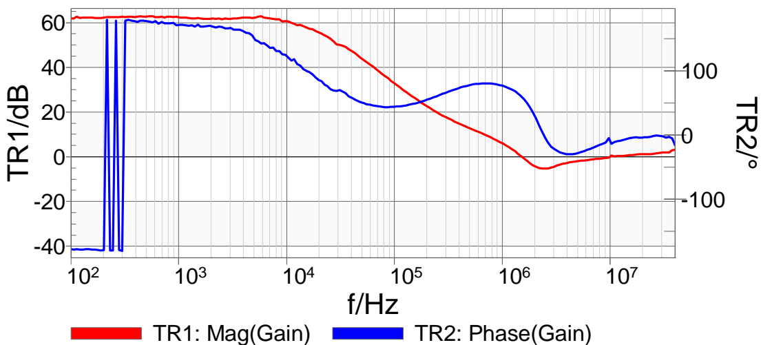
Figure 3 – Bode Plot of LM317 test circuit
