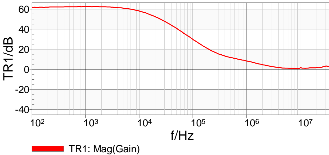
Figure 11 – PSRR of LM317 test circuit
