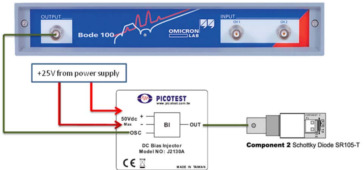
Figure 21 – DC Bias Injector connections to the Bode100 and Component 2 board
