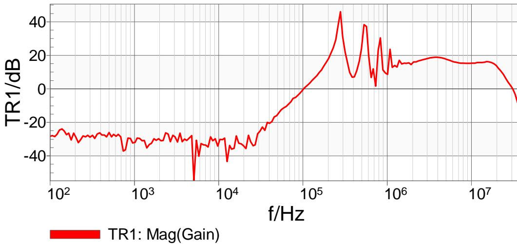
Figure 18 – Crosstalk measurement shown as a voltage gain on the output of the TLV2217 test circuit as a result of current perturbations on the LM317 test circuit.
