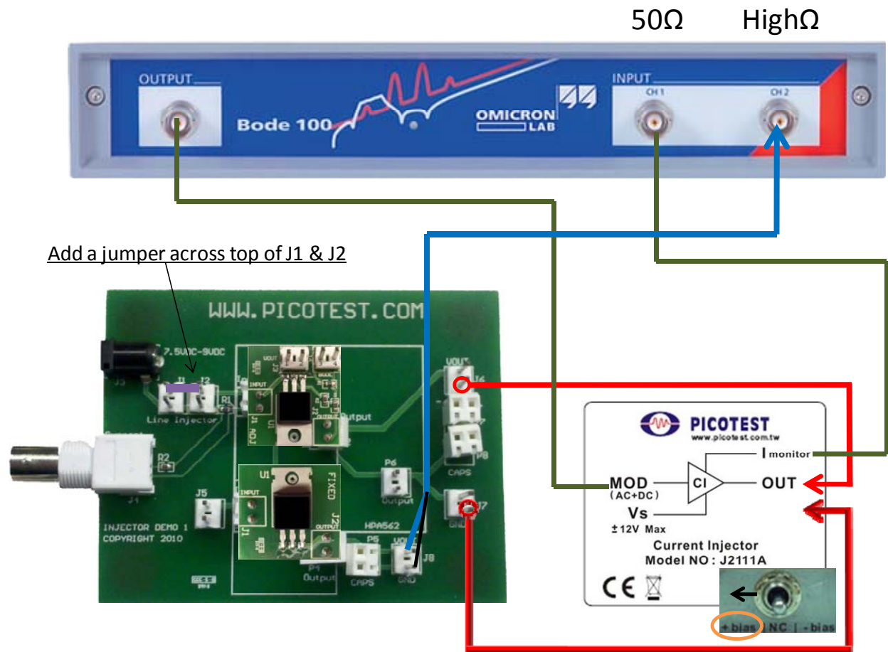
Figure 17 – Current Injector and board connections to the Bode100
