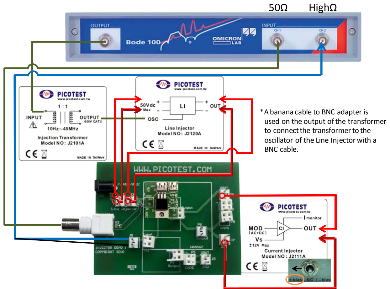
Figure 19 – Line Injector and board connections to the Bode100
