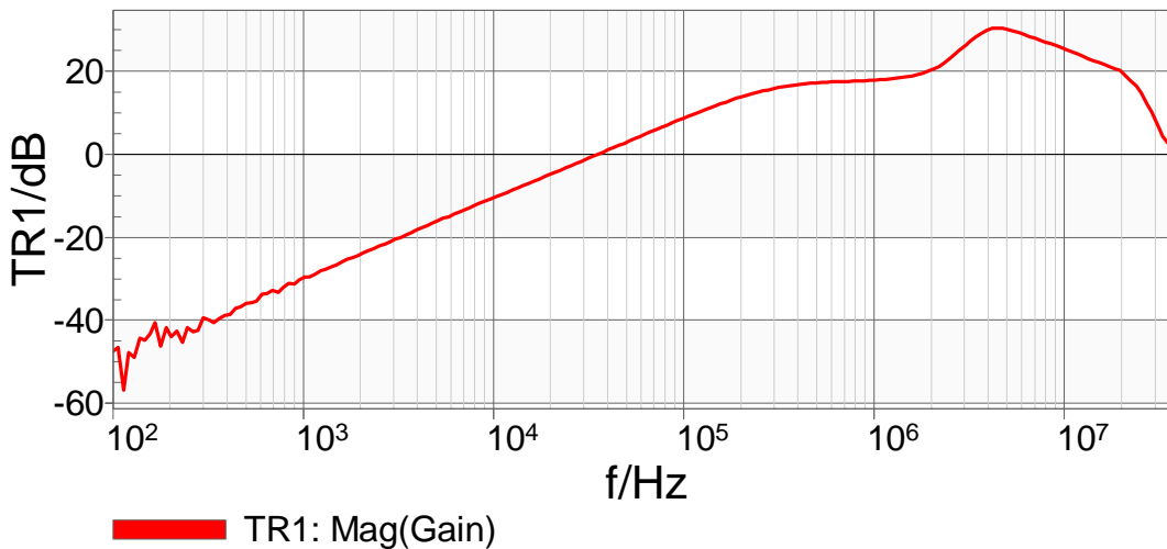
Figure 13 – Output impedance plot of the LM317 test circuit
