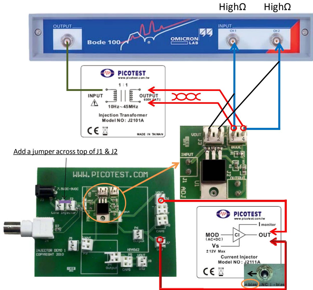
Figure 2 –Bode measurement connection diagram.
