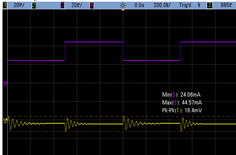
Figure 7 – LM317 output voltage response (Ch1) to load step (Ch3) – 200us time base
