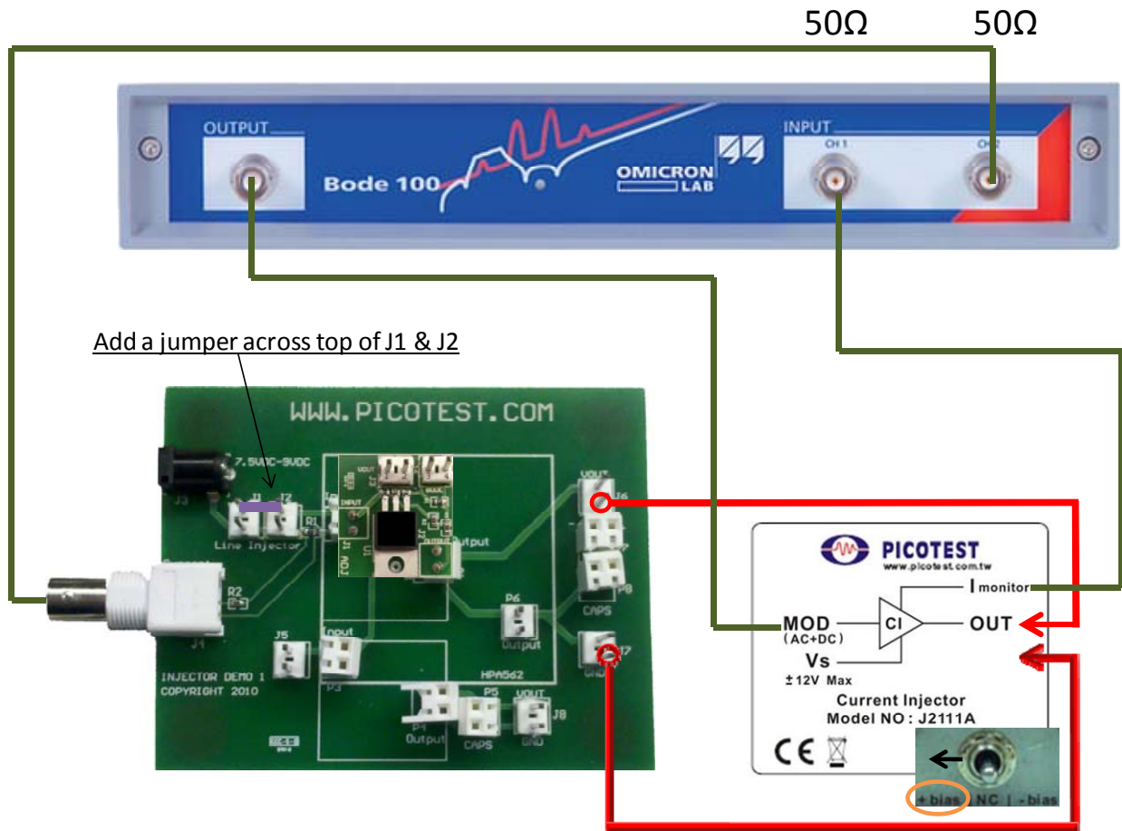
Figure 15 – Current Injector and board connections to the Bode100
