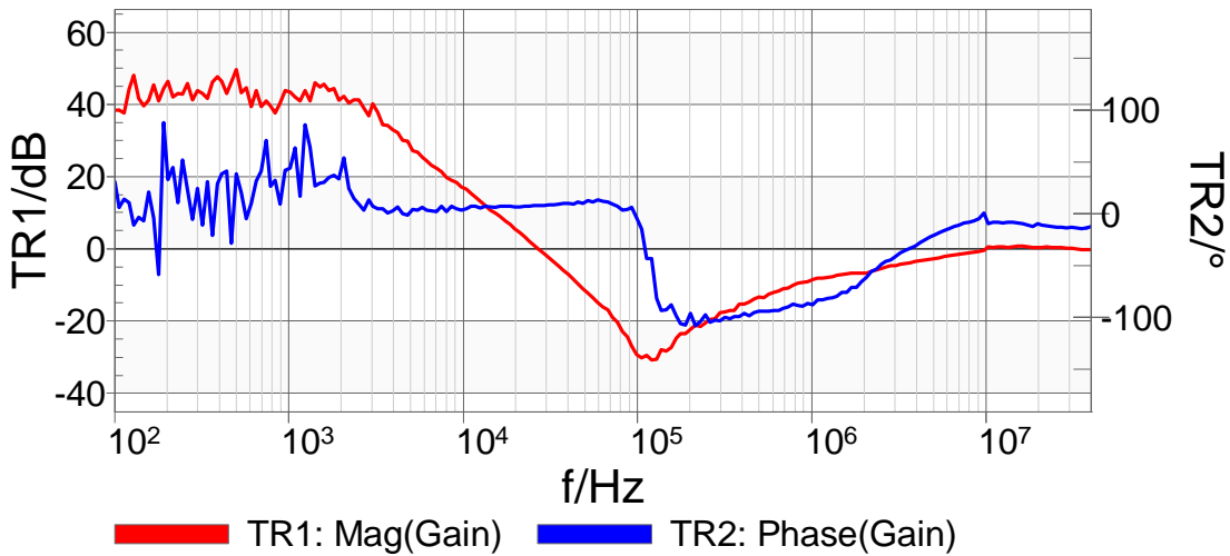
Figure 5 – Correct Bode plot of LM317 test circuit. Signal injection level is at -45dBm
