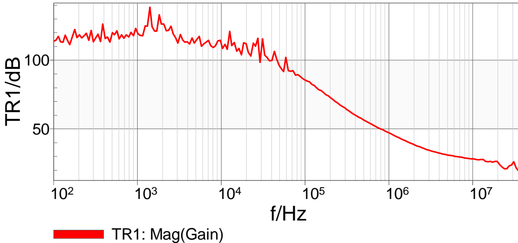
Figure 20 – Input impedance of the LM317 test circuit
