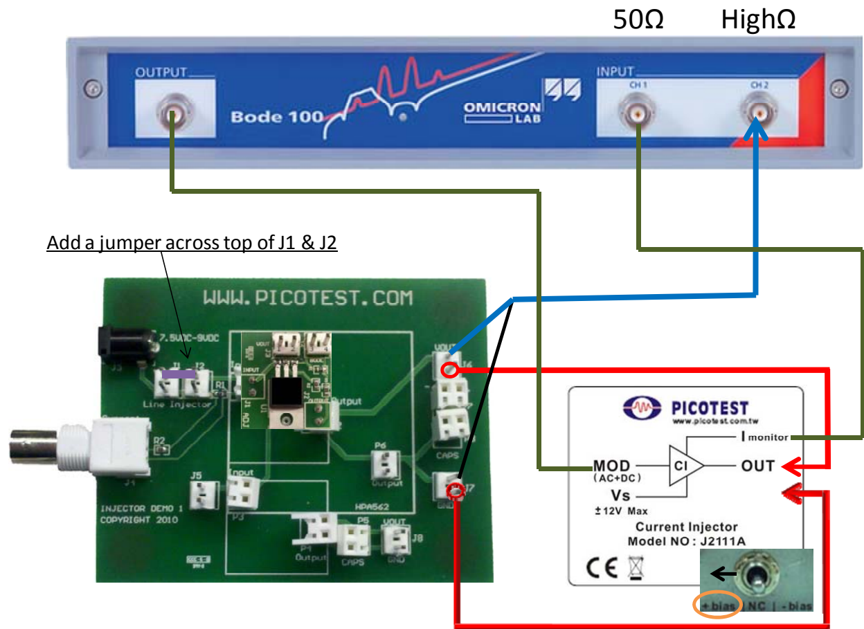
Figure 12 – Output impedance connection diagram
