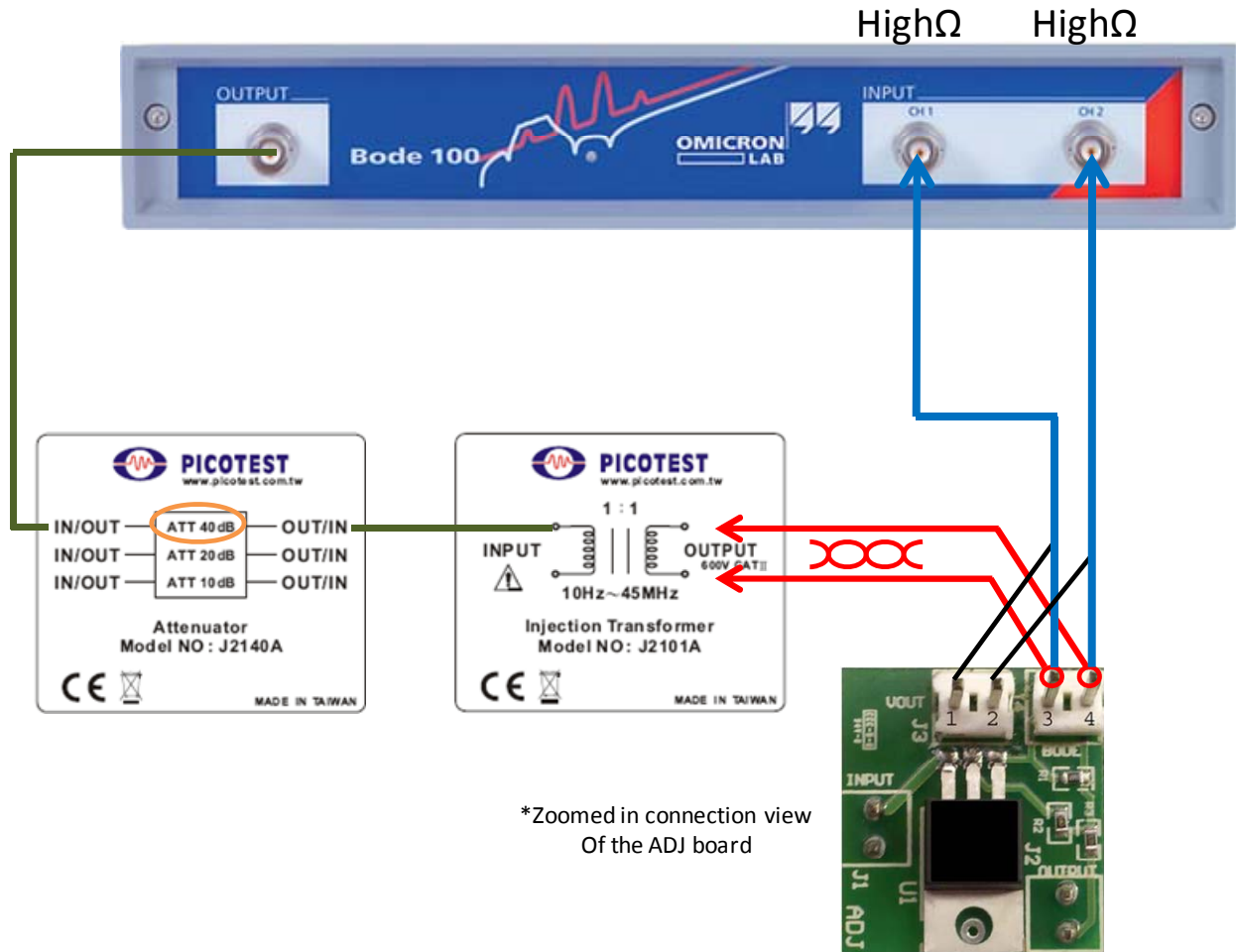
Figure 4 – LM317 to Bode100 connection with the addition of the 40dB Attenuator
