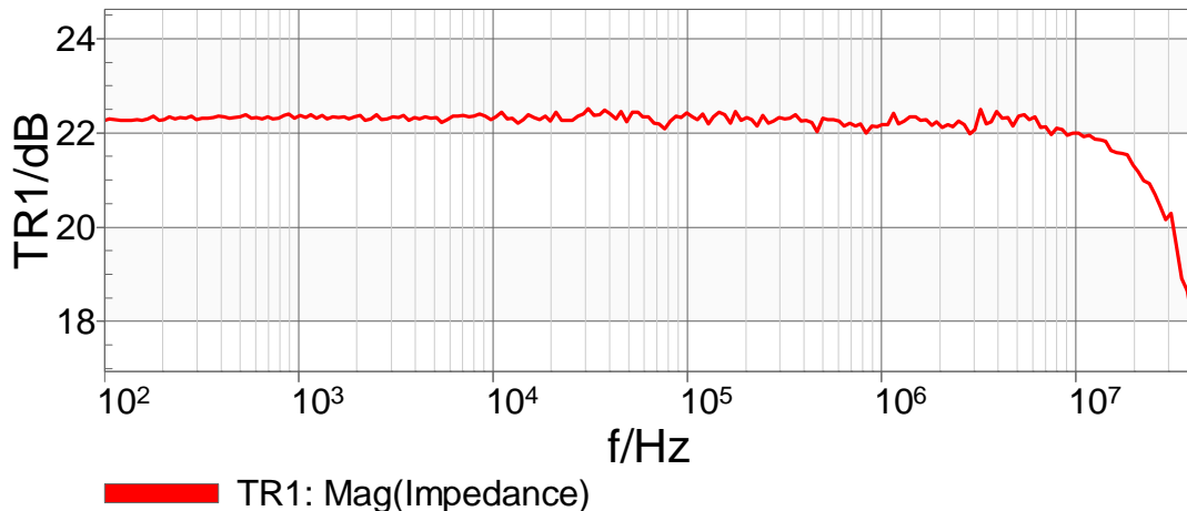
Figure 22 – Impedance of the SR105-T Schottky Diode
