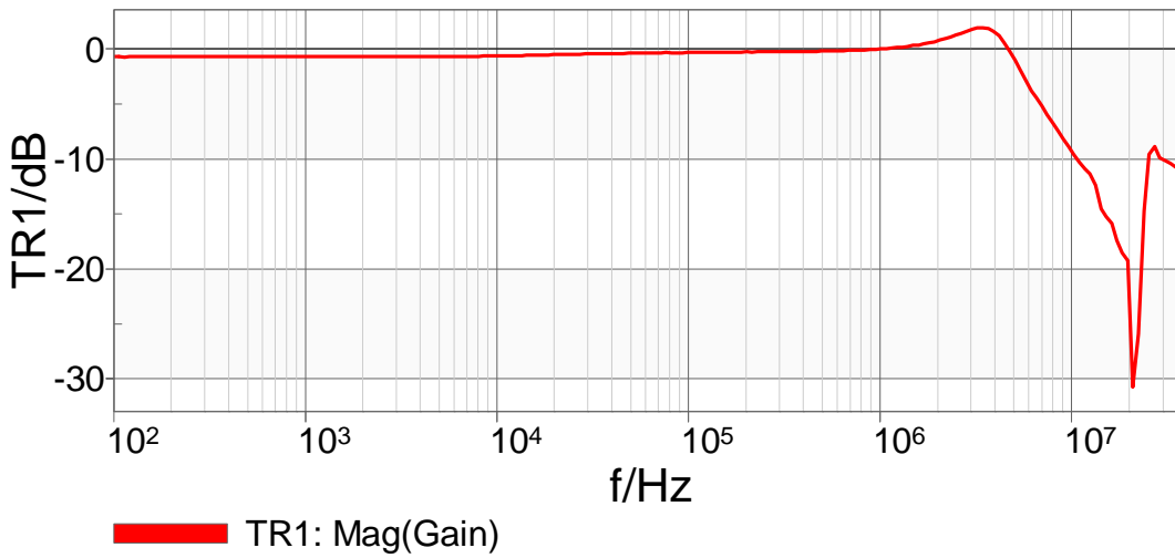
Figure 16 – Reverse transfer plot of the LM317 test circuit
