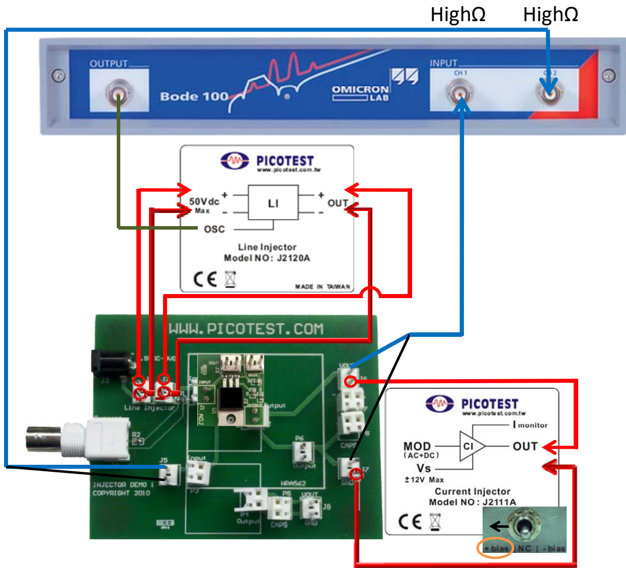
Figure 10 – PSRR connection diagram
