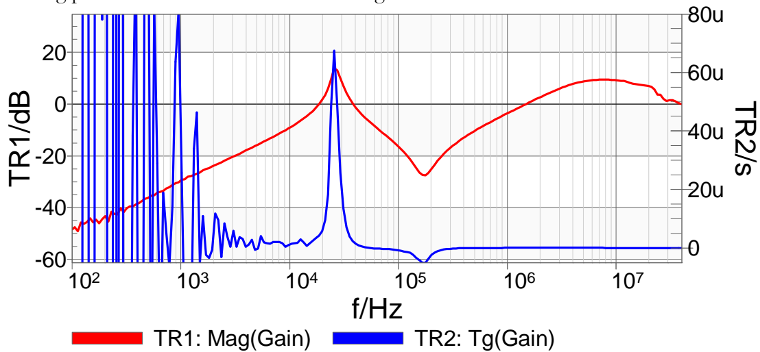
Figure 14 - Output impedance and group delay plot of the LM317 test circuit
