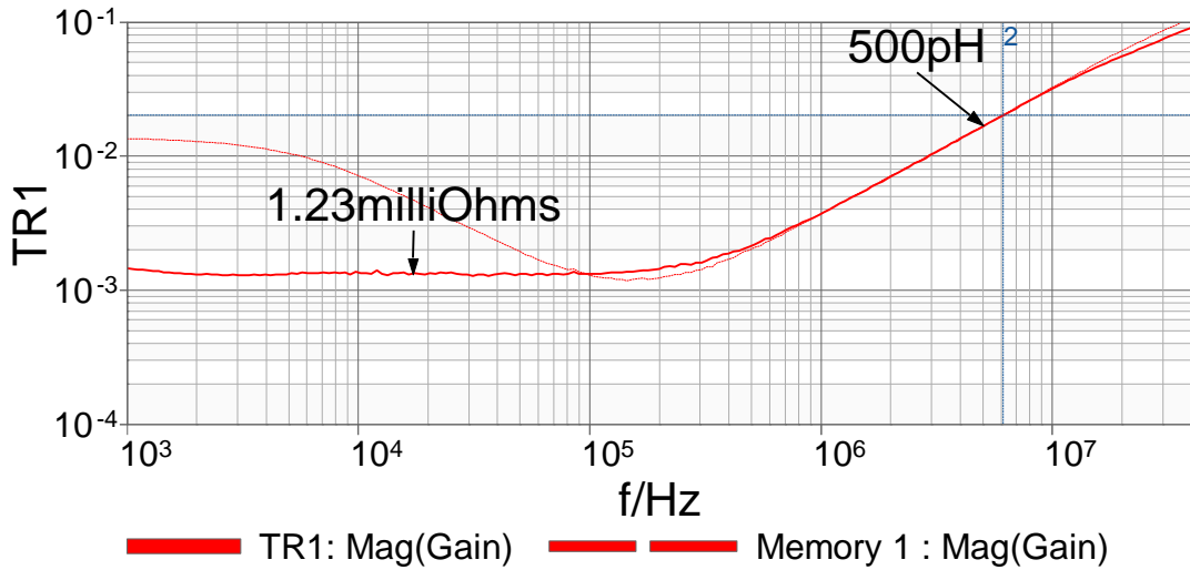
Figure 22: Impedance measurement of a 1mΩ resistor with and without the J2102A common mode transformer using the OMICRON Lab Bode 100.
