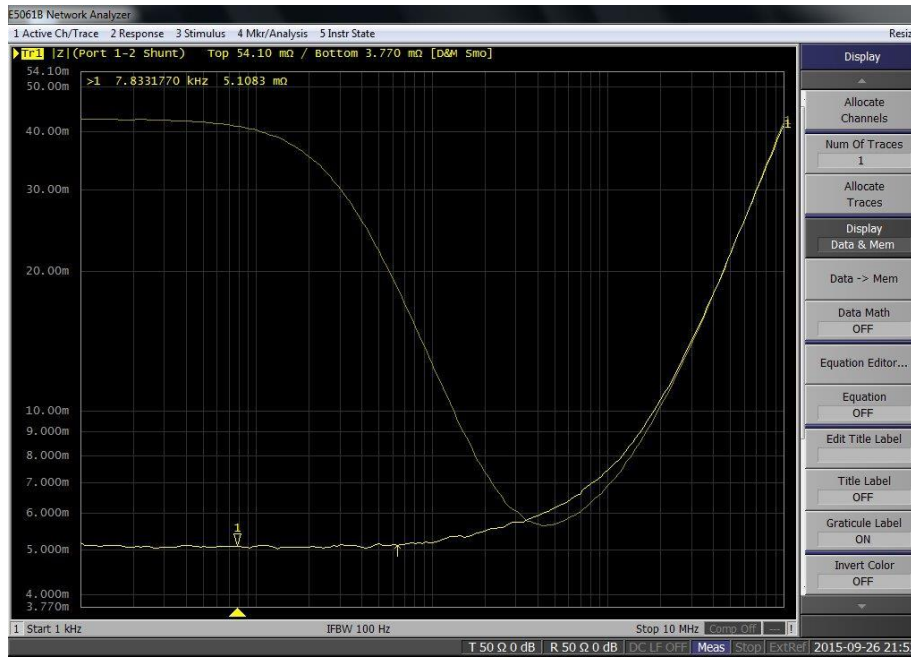
Figure 23: Impedance measurement of a 5mΩ resistor with and without the J2102A common mode transformer using the Keysight E5061B.
