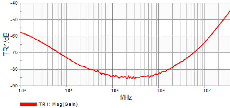
Figure 21: Frequency response of the J2102A.
