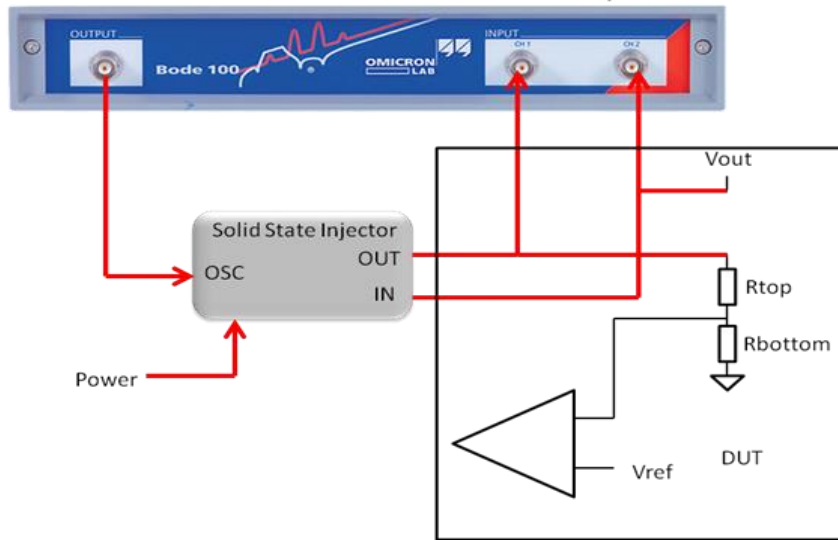
Figure 8 Solid State Injector Connections for stability measurements.
