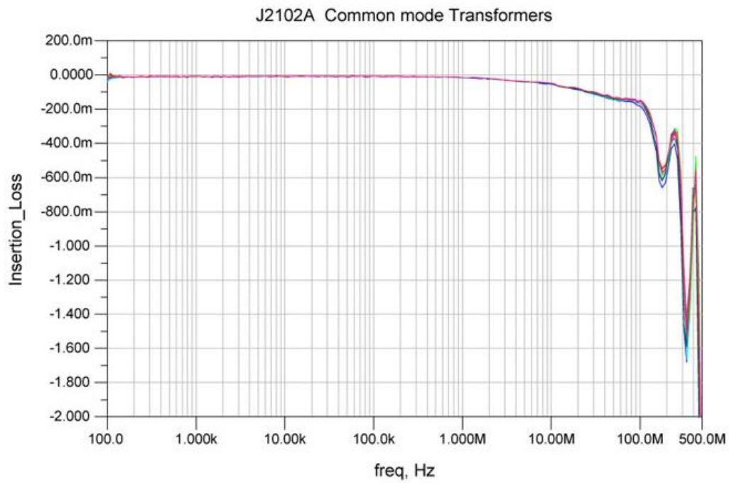
Figure 25: J2102A Insertion Loss Graph.
